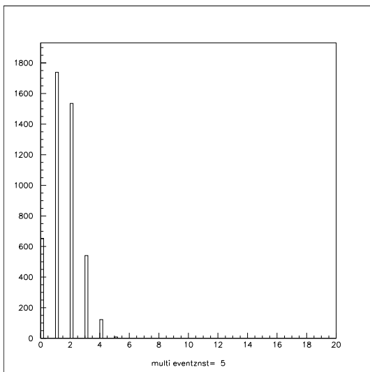
図 0.7 neutron counter が 4 つ (thr6.0MeV)
