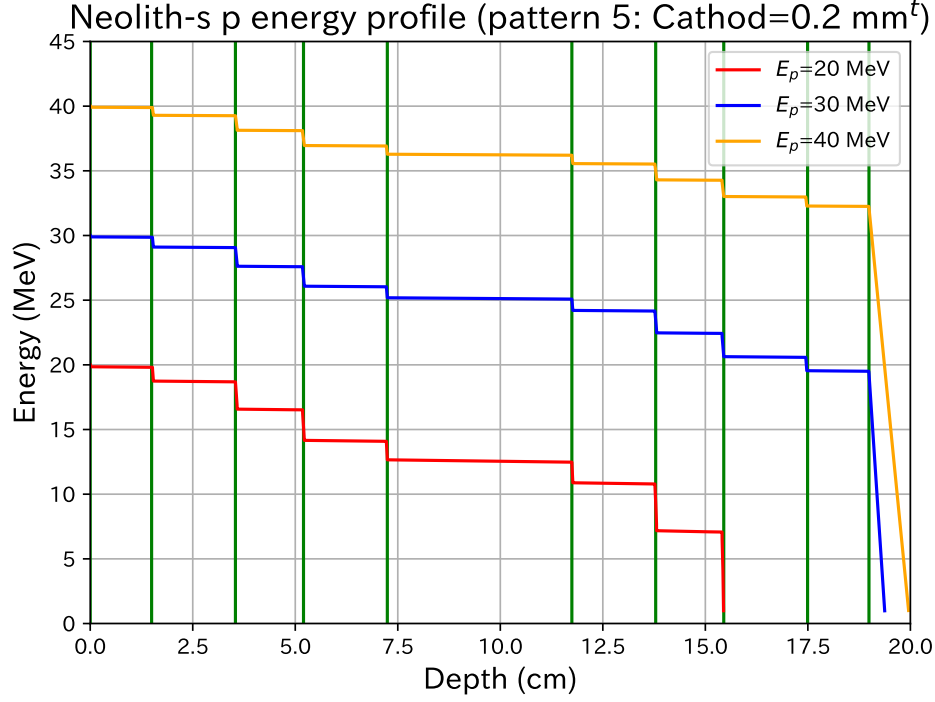
Figure 1: Energy development of protons with energies of 20, 30, and 40 MeV inside the Neolith tracking sections and the rear catcher plastic scintillator. Cathode thickness is 0.2 mm.
