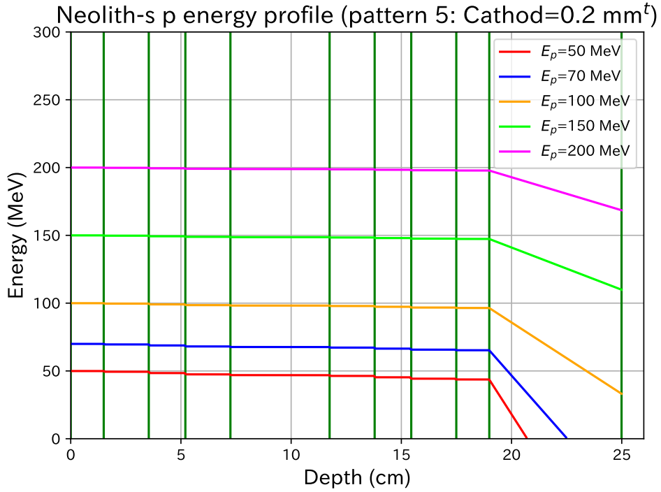
Figure 2: Same as Fig. 1 but for proton energies of 50, 70, 100, 150, and 200 MeV. Cathode thickness is 0.2 mm.
